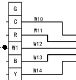
Outdoor Terminal Strip
