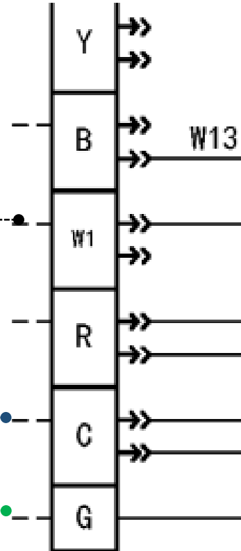
Indoor Terminal Strip
